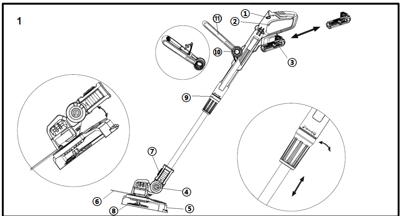
Figure 1: Grass trimmer
